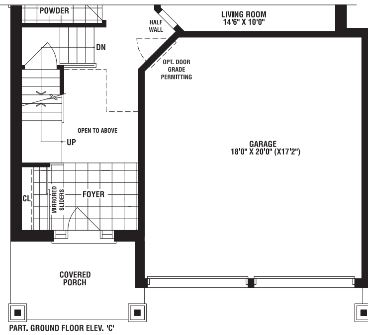
PART. GROUND FLOOR ELEV. 'C'
