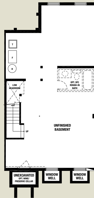
UNFINISHED BASEMENT ELEV 'A' INTERIOR CONDITION
