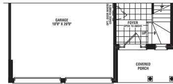
PART. GROUND FLOOR ELEV. 'C'
