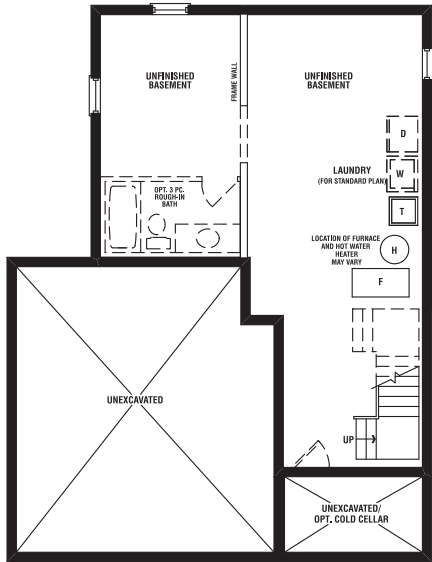
BASEMENT ELEV. 'A' & 'C'
