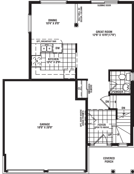
GROUND FLOOR ELEV. 'A'
