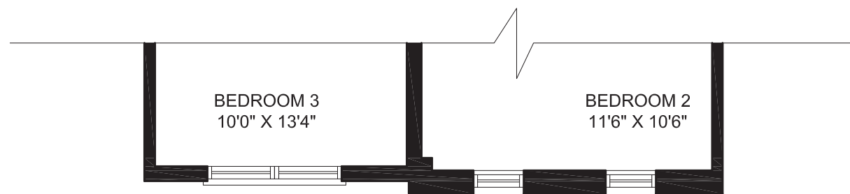
PARTIAL SECOND FLOOR STYLE B
