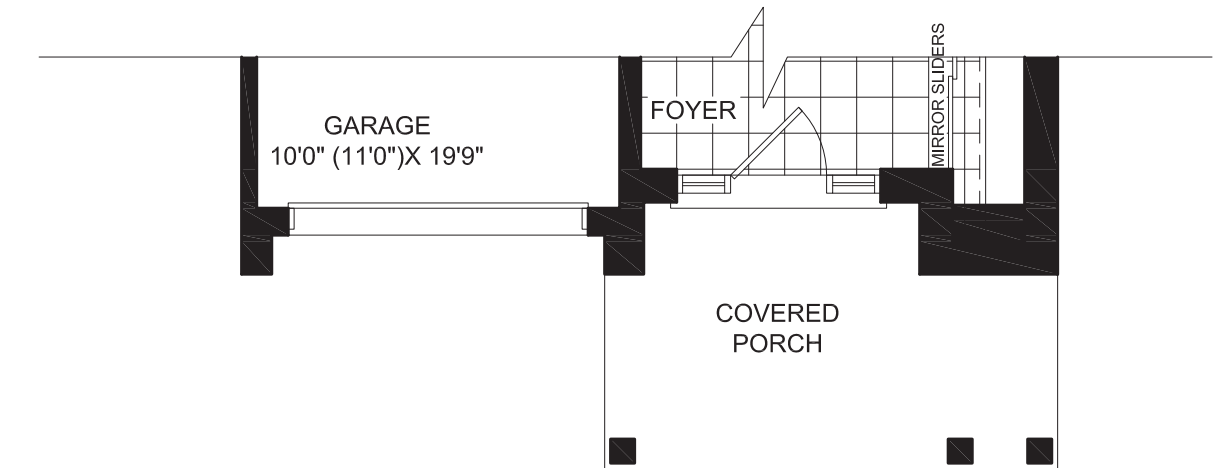
PARTIAL GROUND FLOOR STYLE B
